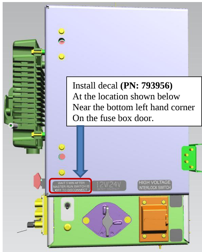
FIGURE 1A: DECAL INSTALLED ON FUSE BOX DOOR
