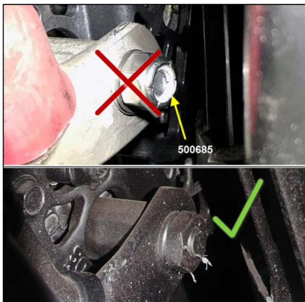
FIGURE 72: HARDWARE TO USE WITH EARLY VERSIONS
