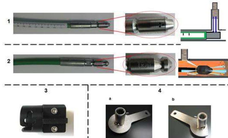
Figure 12. Special tool set VAS6825.
