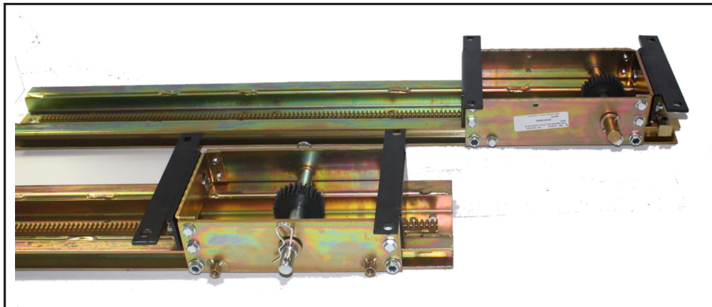
Top: New bolt-on side plate. Bottom, original weld-on side plate. The weld-on side plate will be obsoleted.
