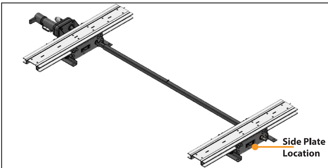
Example of side plate location on a slide-out system.
