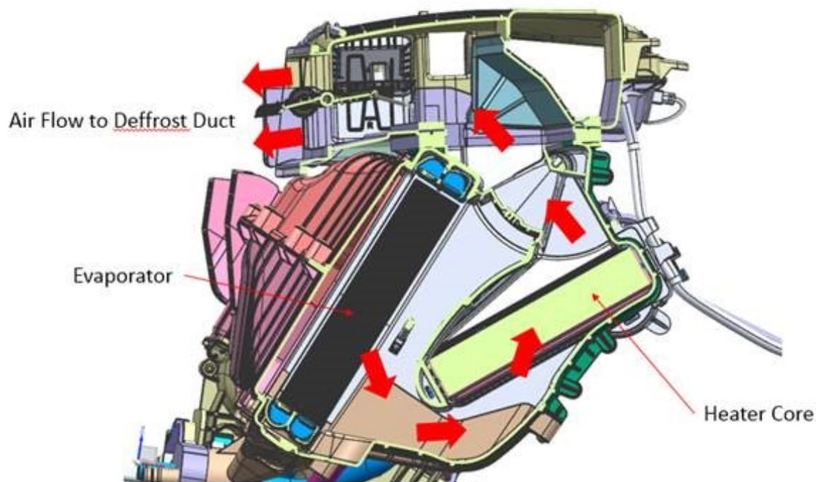
DEFROST MODE – FULL HOT, OSA (Outside Air)
