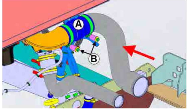
FIGURE 97: CONNECTION AT THE TURBO OUTLET ELBOW
