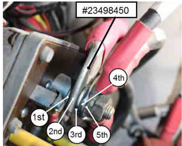
FIGURE 142: ON THIS PICTURE, CABLE #23498450 LUG IS IN SECOND (2 ND ) POSITION BECAUSE IT WAS LIKELY TO RUB ON THE HEAD OF ONE OF THE FOUR SCREWS.
