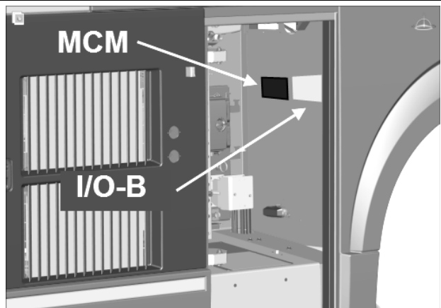
FIGURE 147: MAIN POWER COMPARTMENT
