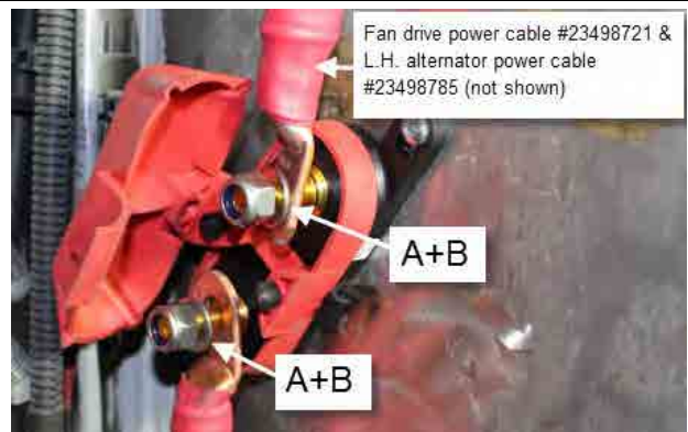
FIGURE 144: TAKE NOTE THAT THE 300A FUSE IS NOT PRESENT ON THE PICTURE ABOVE BUT IT SHOULD BE INSTALLED AT THIS STEP
