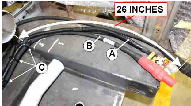
FIGURE 87 A: FAN TO RJB INTERFACE” HARNESS #23488790 B: FAN DRIVE POWER CABLE C: NYLON TIES #504016 (23x approx.)
