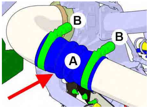
FIGURE 92: CONNECTION AT THE ENGINE INTAKE ELBOW
