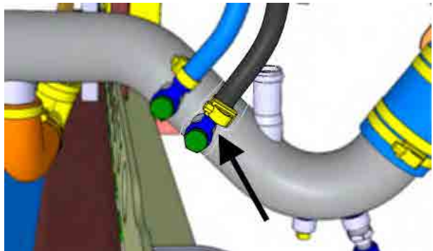
FIGURE 70: DEF INJECTOR COOLANT LINE RETURN HOSE
