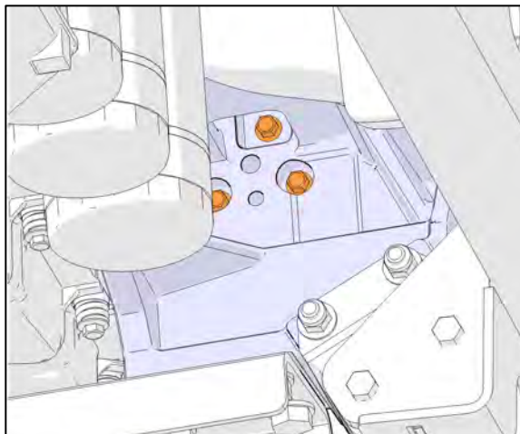
FIGURE 44: IDLER / TENSIONER ASSEMBLY MOUNTING SCREWS
