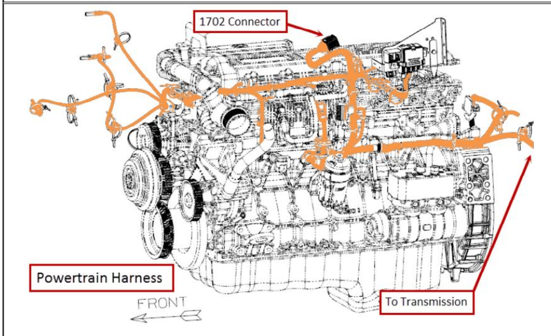
Figure 7 - Powertrain Harness
