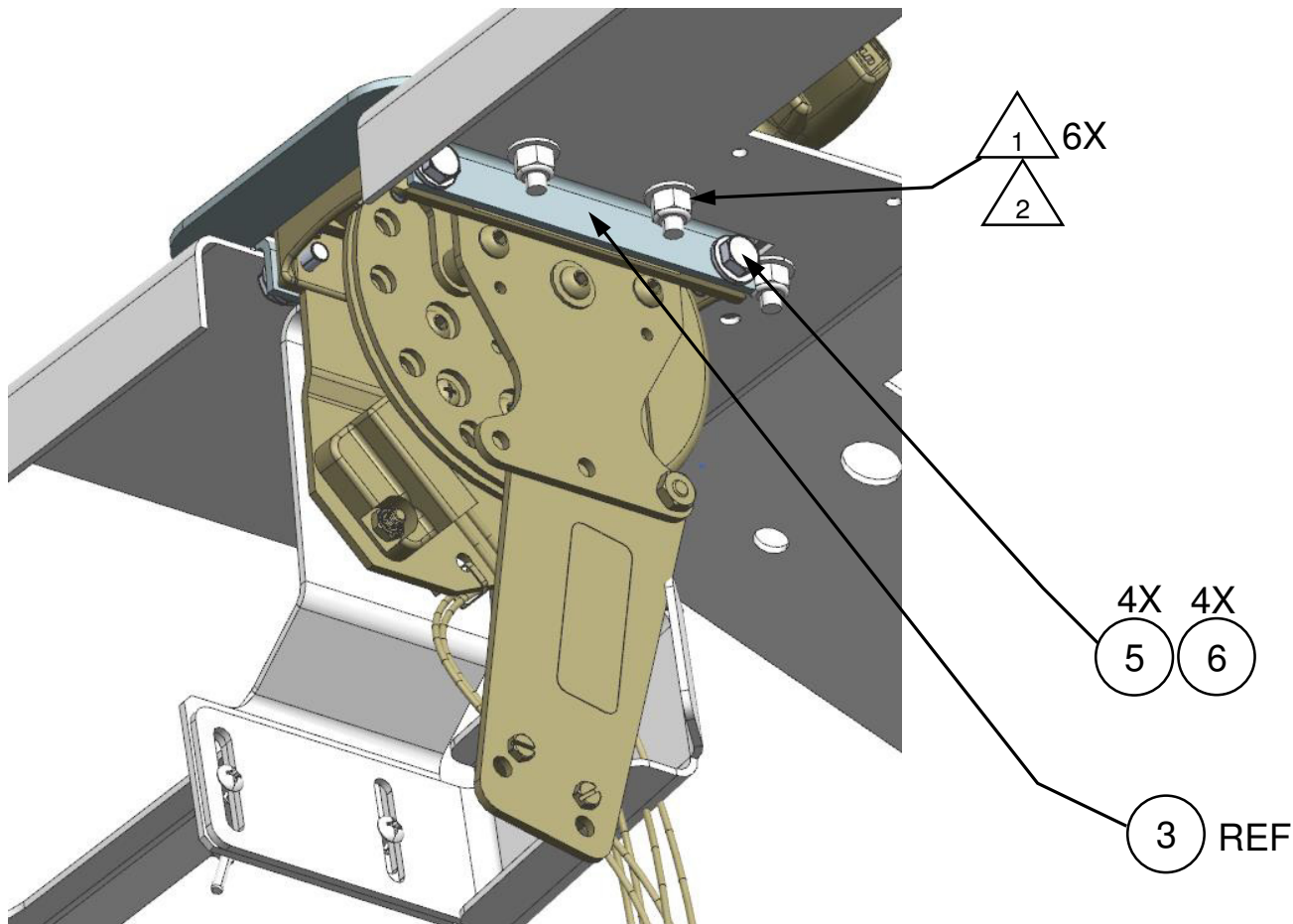
VIEW B
