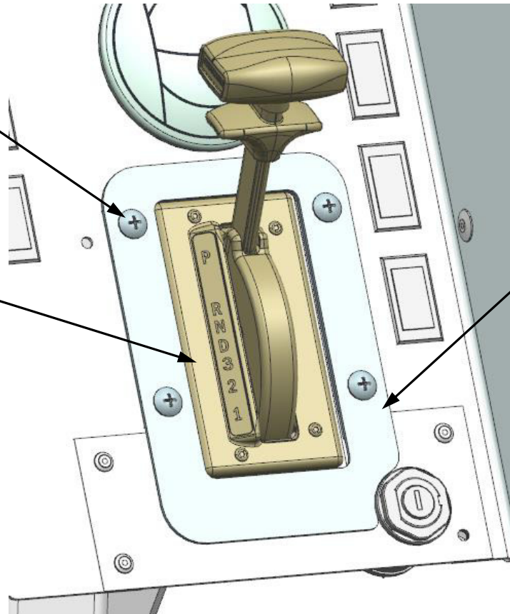
VIEW A
