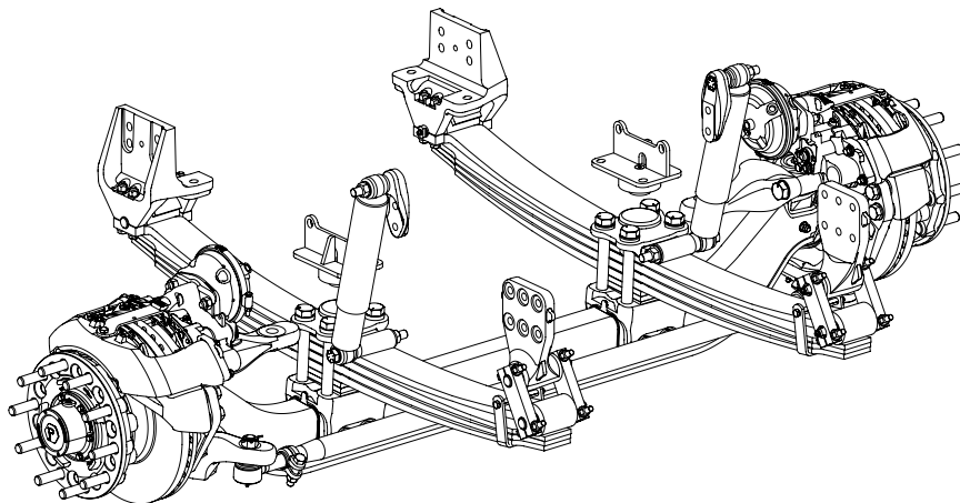
STEERTEK NXT High Capacity with Air Disc Brakes
