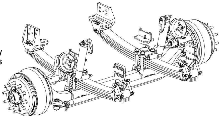
STEERTEK NXT High Capacity with Drum Brakes
