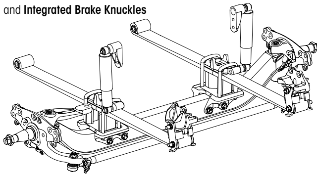
STEERTEK NXT axle with International Truck 2-leaf mechanical suspension
