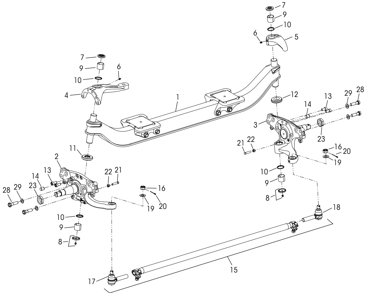
STEERTEK NXT Integrated Axle Spring Seat with Shock Absorber Lug
