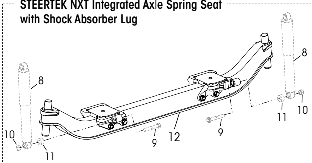
STEERTEK NXT with Standard Knuckle Assembly
