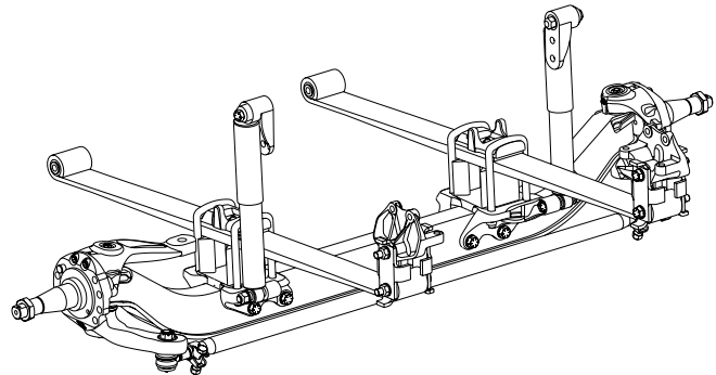
SOFTEK MONOLEAF with STEERTEK NXT axle
