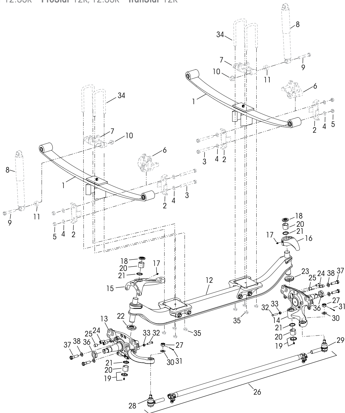
STEERTEK NXT Integrated Axle Spring Seat with Shock Absorber Lug
