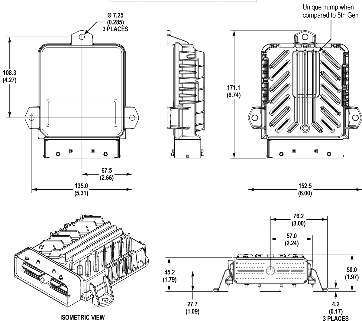
Figure 2. 6th Generation Controls Hardware
