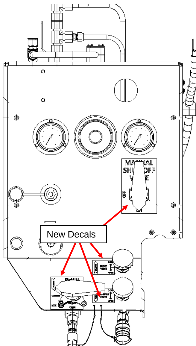
Figure 1: Install new decals as shown
