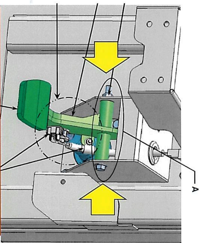
DETAIL A - EXPLODED FOR CLARITY
