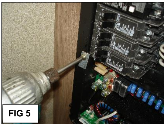
FIG 5: Remove one screw holding the breakers in place. FIG 6: Remove the 20/15A breaker which is located at the bottom of the row.
