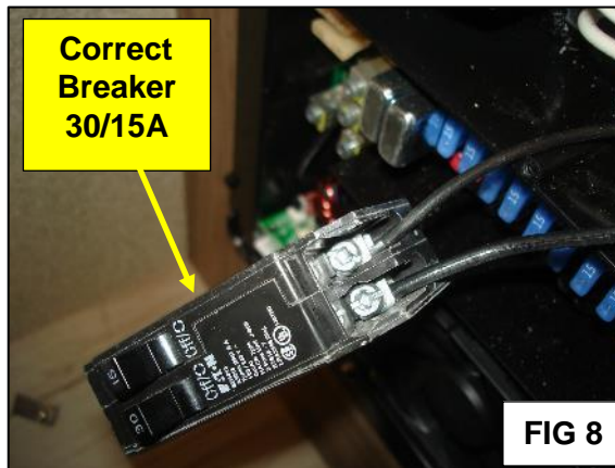
FIG 7: Remove both wires from the breaker using the screw gun or a Phillips screwdriver. FIG 8: Replace the 20/15A breaker with a 30/15A and attach the heavier gauge wire to the 30A side. Smaller gauge wire attaches to the 15A side.
