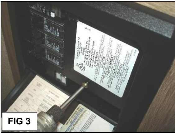
FIG 3: Remove one screw holding the cover to the breaker panel. FIG 4: Cover will pop off, revealing the breakers.
