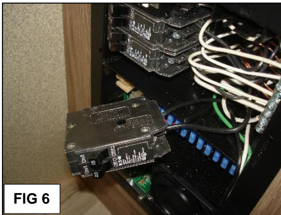
FIG 5: Remove one screw holding the breakers in place. FIG 6: Remove the 20/15A breaker which is located at the bottom of the row.
