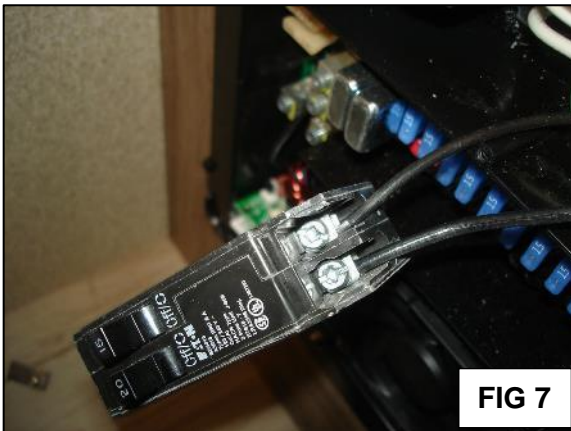
FIG 7: Remove both wires from the breaker using the screw gun or a Phillips screwdriver. FIG 8: Replace the 20/15A breaker with a 30/15A and attach the heavier gauge wire to the 30A side. Smaller gauge wire attaches to the 15A side.
