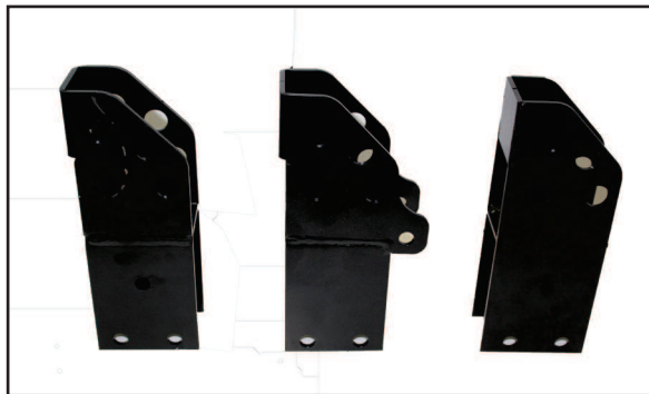
From left are current bike rack brackets 243632 and 369559 and new bracket 719822.
