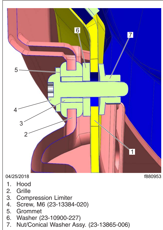
Fig. 2, Grille Fasteners
