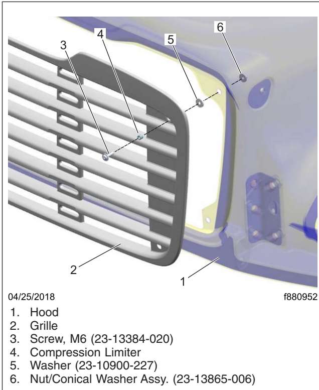
Fig. 1, Grille Installation
