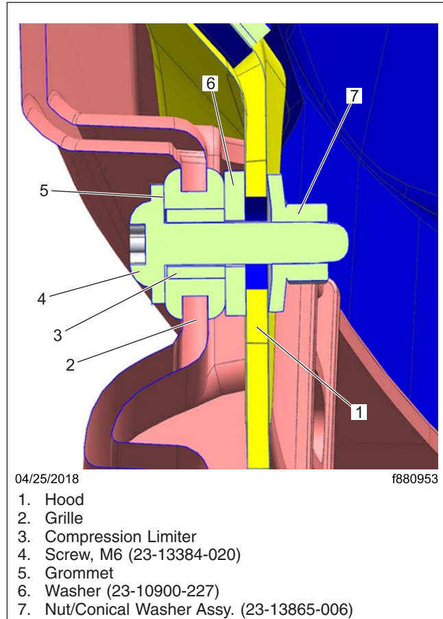
Fig. 2, Grille Fasteners
