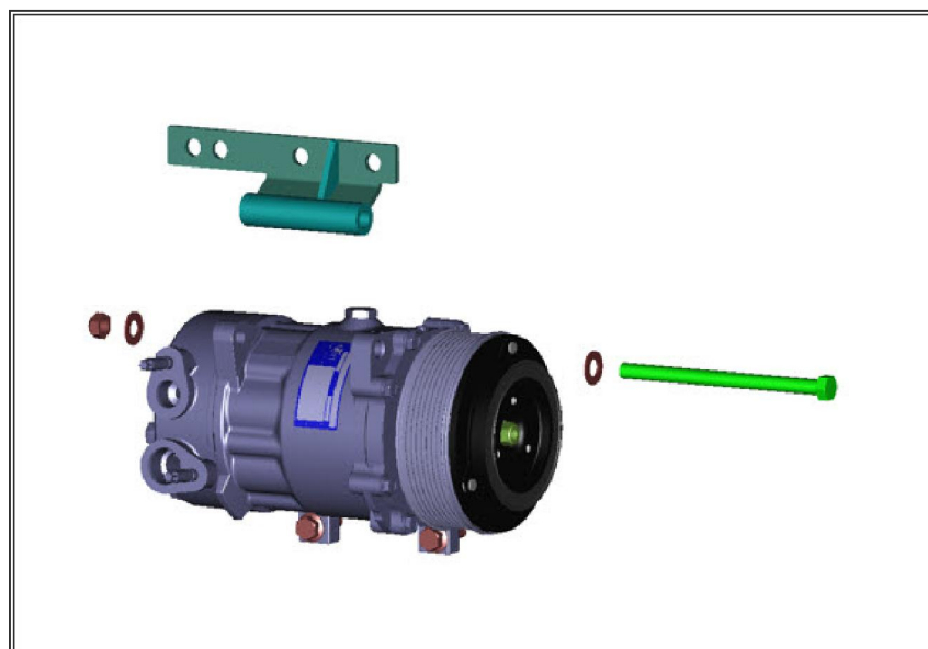
Figure #2: Proper torque procedure
