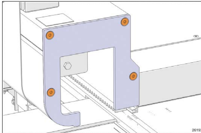
FIGURE 2: EXTRUSION END CAP
