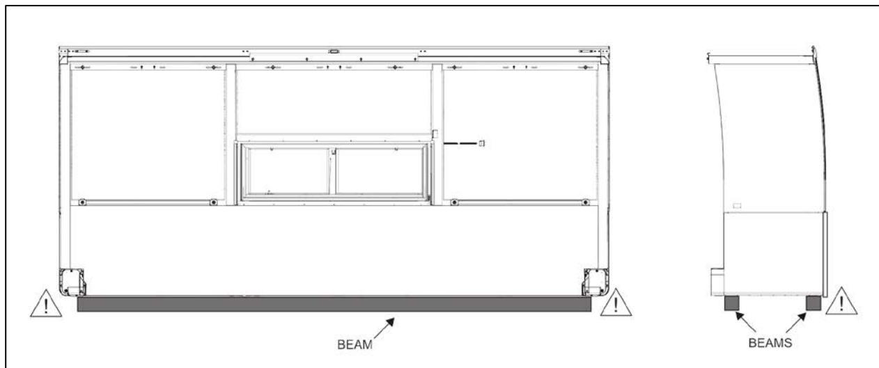
FIGURE 1: BEAM PLACEMENT
