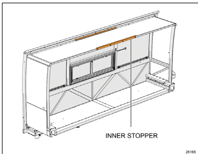
FIGURE 4: UPPER INNER STOPPER
