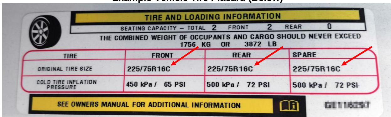
Example Vehicle Tire Placard (Below)
