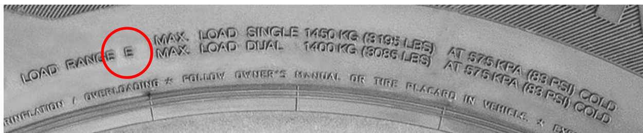
Load Range, Max Load and Pressure Specifications for the Tire Photo Shown Above
