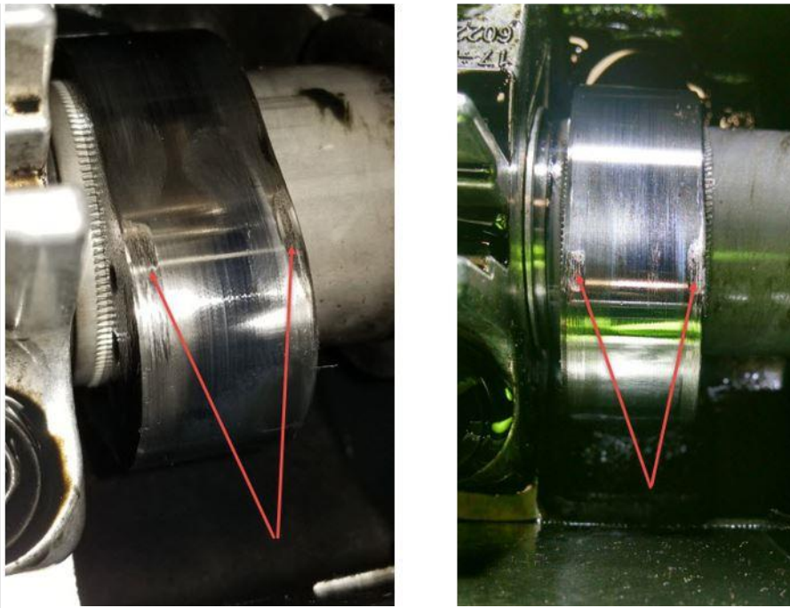
Figure #3: DO NOT Reuse - Impact Damage
