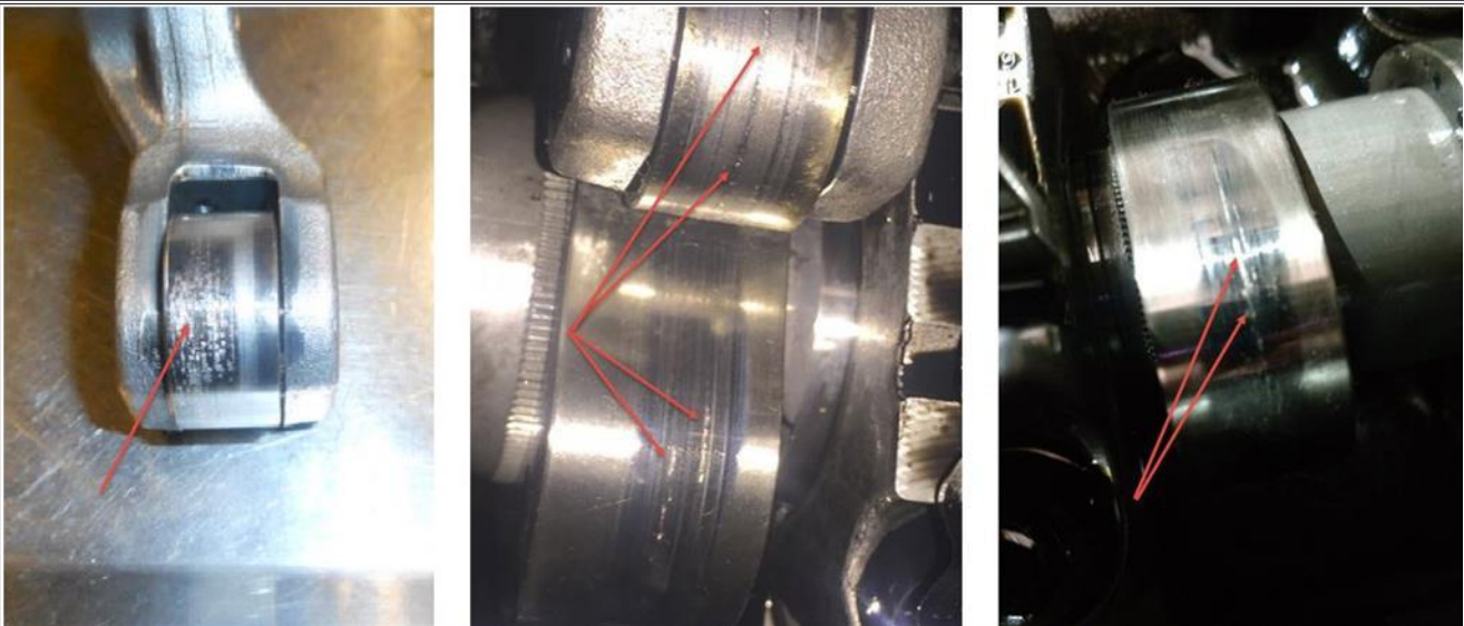
Figure #2: DO NOT Reuse - Macropitting and Spalling
