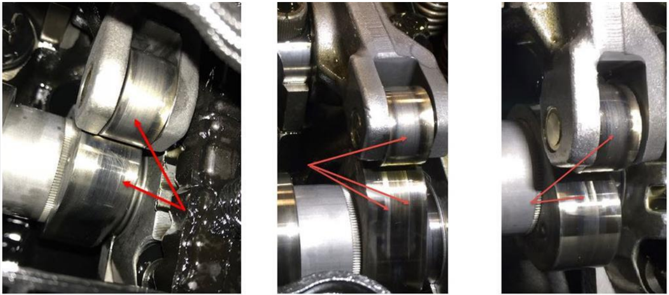
Figure #1: USE AGAIN - Roller frosting and visual lines
