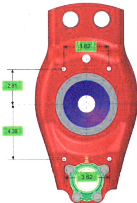
Figure 1: Old mounting hole location
