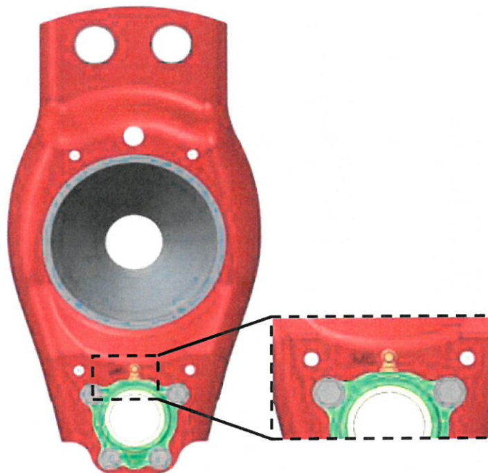
Figure 4: Brake spider with "M6" marking
