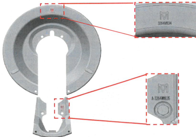
Figure 3: Part numbers of new dust shield's components
