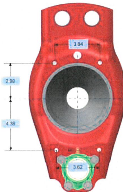
Figure 2: New mounting hole location
