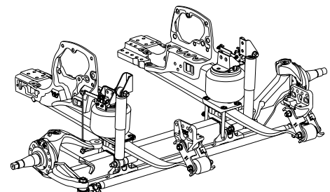
AIRTEK with STEERTEK Axle – Western Star
