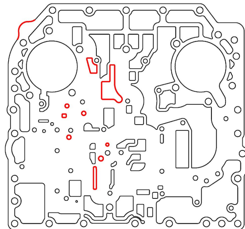
P/N 29557345 (TID B Aluminum Main Valve Body Configuration)
