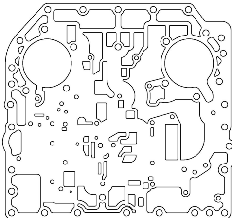
P/N 29546538 (TID A Cast Iron Main Valve Body Configuration)
