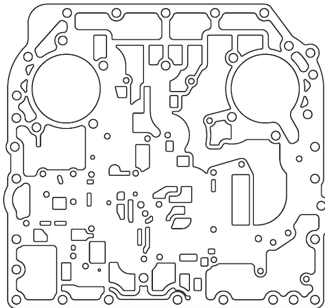
P/N 29542919 (TID 3 or TID A Cast Iron Main Valve Body Configuration)
