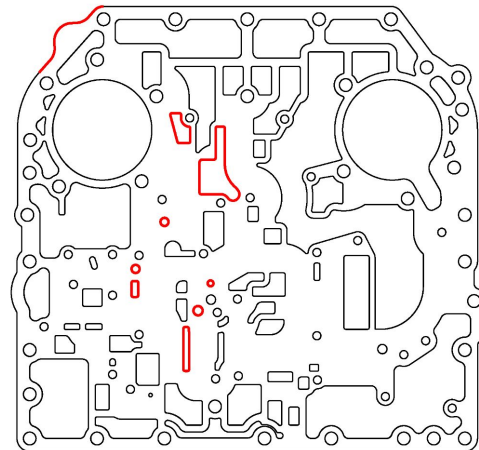
P/N 29557346 (TID B Aluminum Main Valve Body Configuration)
