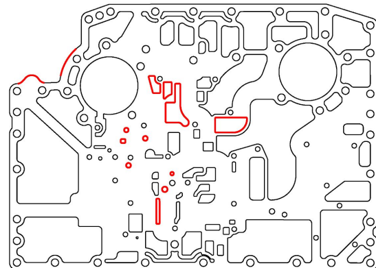
P/N 29557347 (TID B Aluminum Main Valve Body Configuration)
