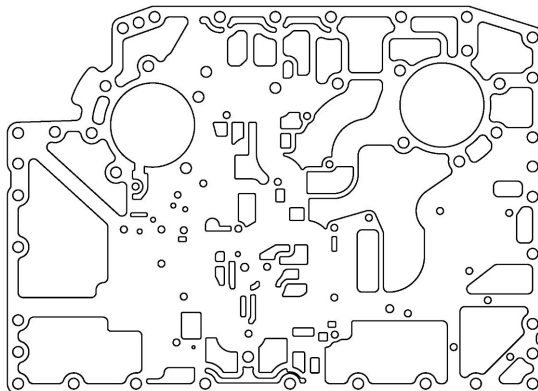
P/N 29546539 (TID A Cast Iron Main Valve Body Configuration)
