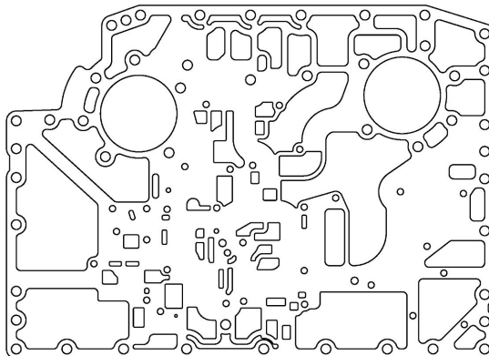
P/N 29542920 (TID 3 or TID A Cast Iron Main Valve Body Configurations)
