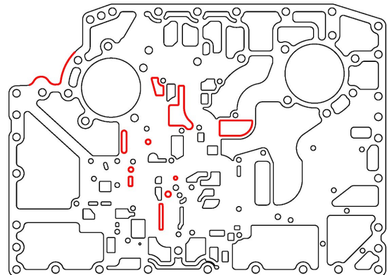
P/N 29557348 (TID B Aluminum Main Valve Body Configurations)
