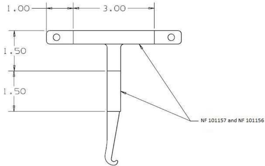
Figure 1: Velcro Location
