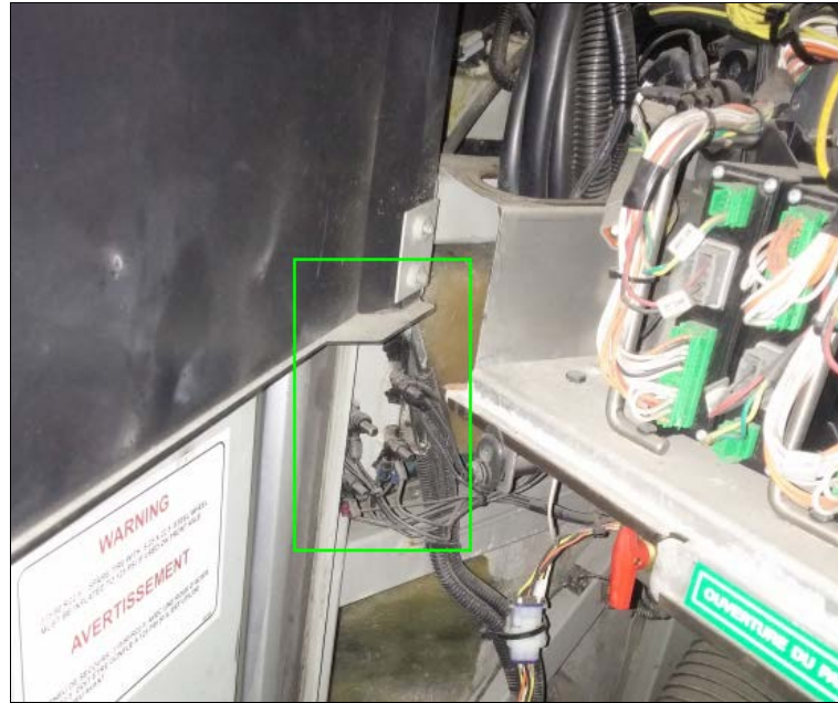
GROUND STUDS LOCATION IN FRONT COMPARTMENT (X3 VEHICLES)
