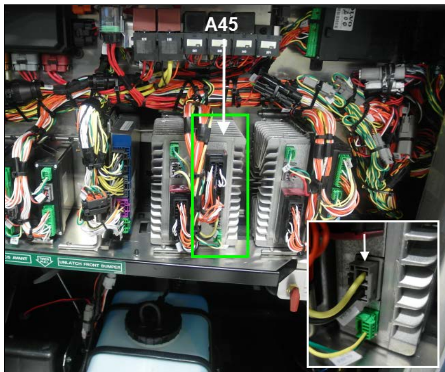
A45 MODULE AND GREY CONNECTOR (12V WAKE-UP)
