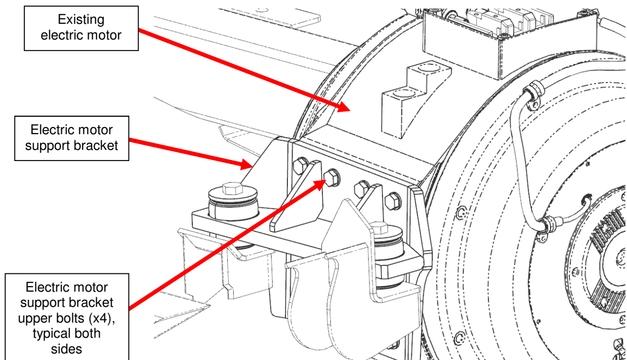
Figure 1: Electric Motor Support Bracket Upper Bolt Locations
