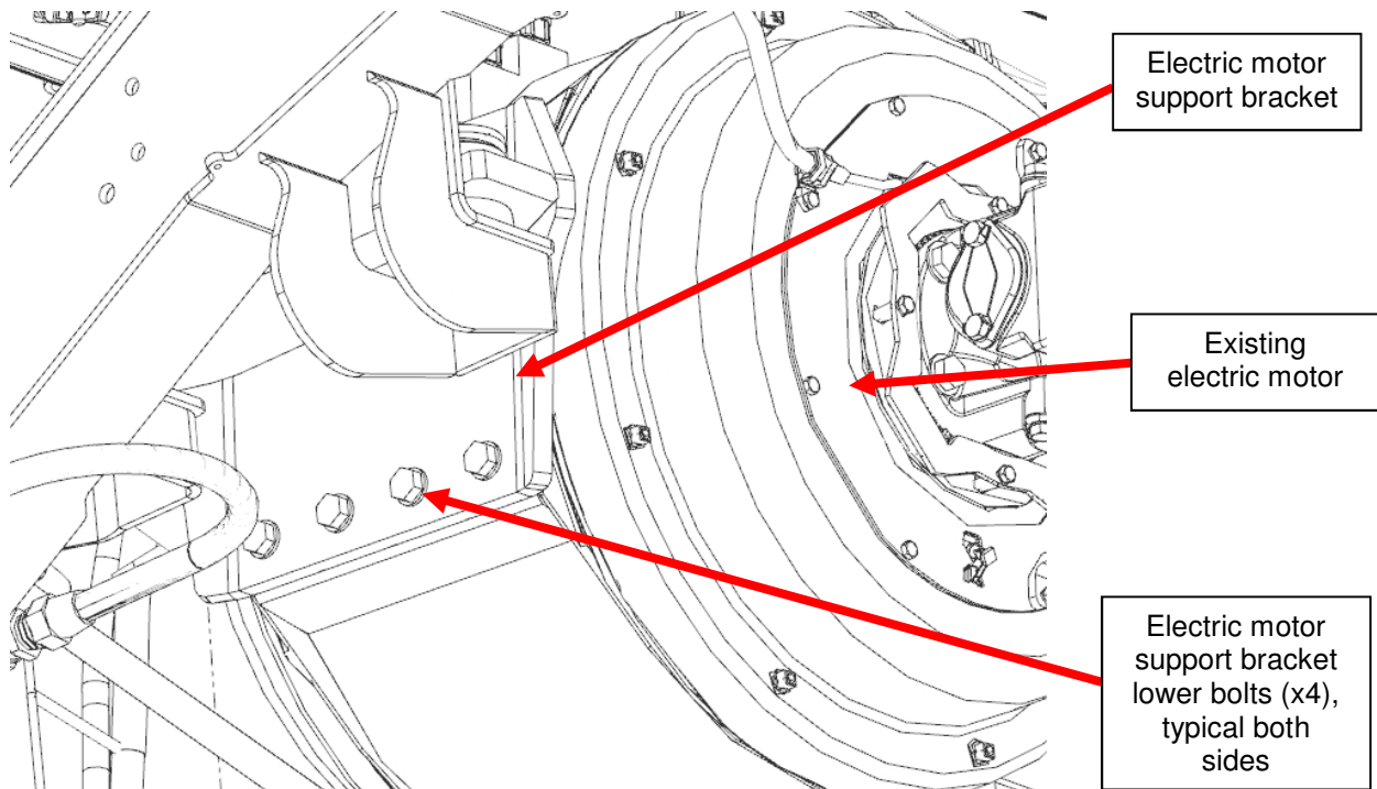
Figure 2: Electric Motor Support Bracket Lower Bolt Locations
