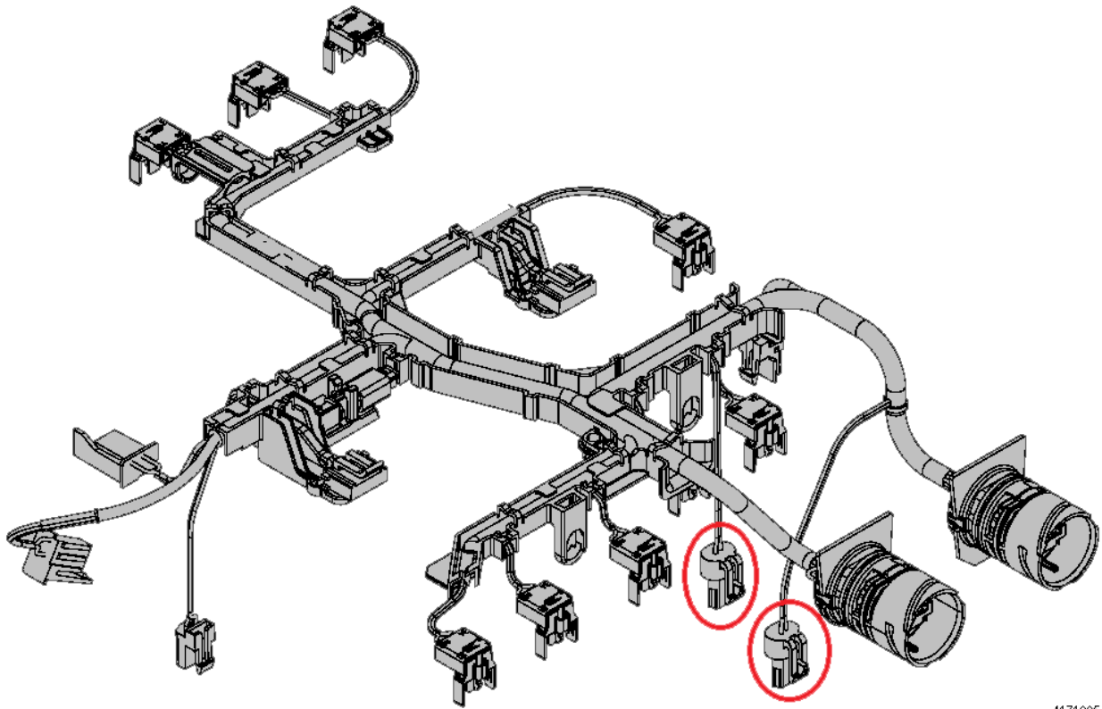
Figure 1. Internal Wiring Harness Speed Sensor Connector Locations
