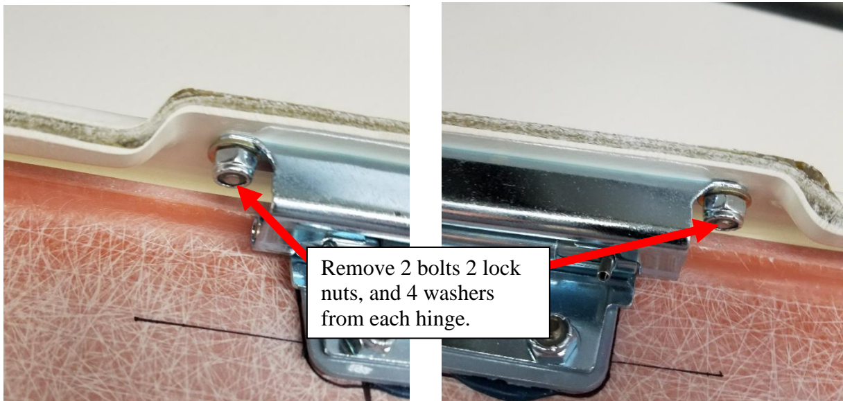
Figure 4: Old air filter door hinge hardware
