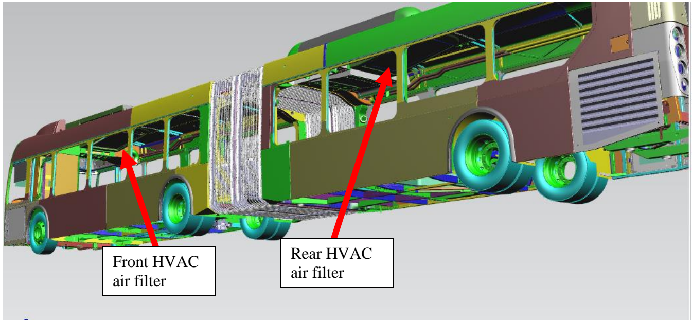
Figure 1: Street side view of bus
