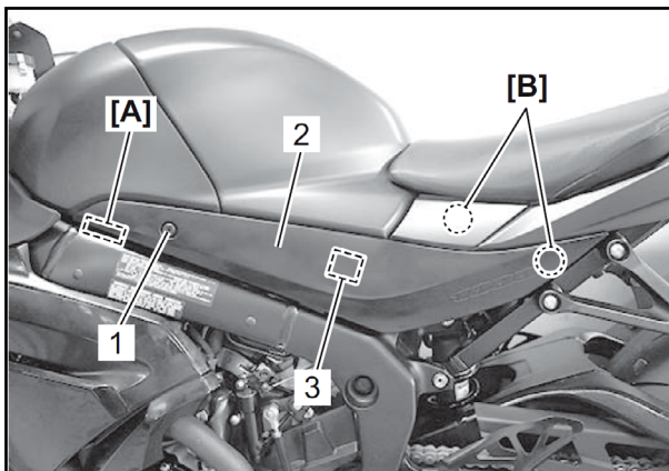
[A] Hooked Point, [B] Bushing, 3 - Velcro
