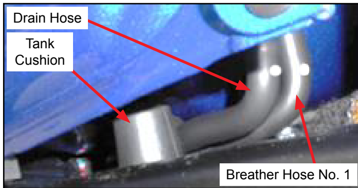
The fuel tank drain hose and breather hose No. 1 are routed to the inside of the tank cushion
