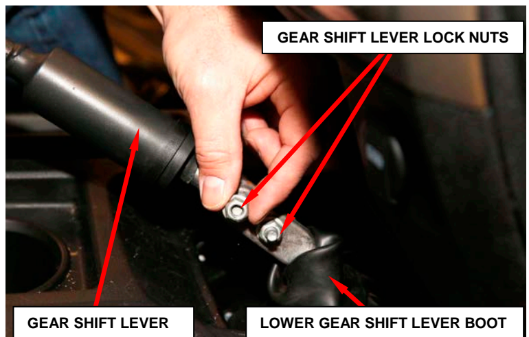
Figure 6 – Lock Nuts
