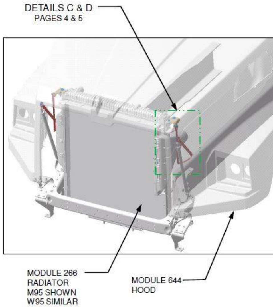
Fig 2: A/C Pressure switch next to strap, with improvement already installed
