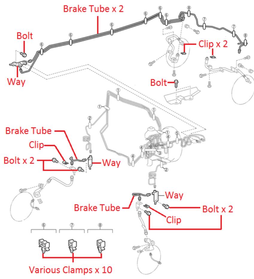
Frame Mounted Brake Lines
