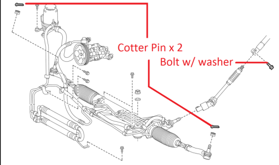
Power Steering
