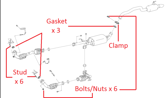
Exhaust System (Parts vary with engine)
