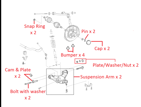
Front End
