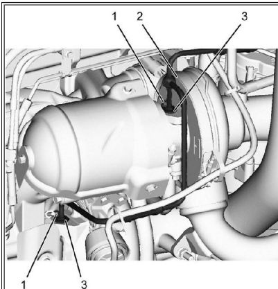
Figure 13: Turbocharger Oil Supply Openings.
