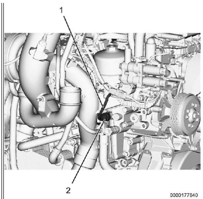
Figure 4: Engine Oil Pressure (EOP) Sensor.
