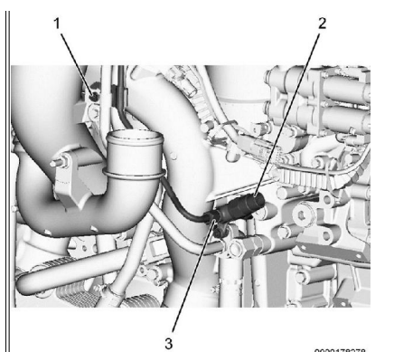
Figure 14: Turbo Oil Supply Tube T-fitting Flare Nut.
