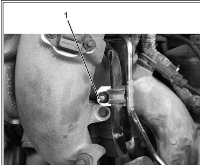
Figure 12: Heater and Cooler Line Bracket Stud Bolt.
