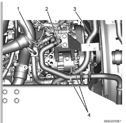
Figure 22: Water Bypass Hose.
