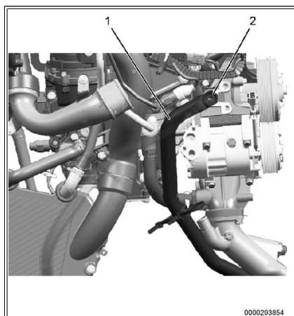
Figure 26: SCR Equipped Water Bypass Hose Replacement.
