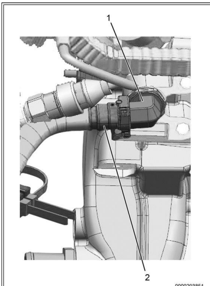
Figure 23: Coolant Deaeration Tank Supply Hose.
