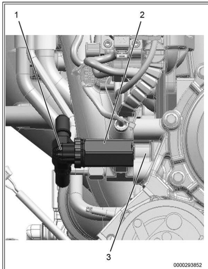
Figure 24: Coolant Deaeration Tank Supply Hose Spacer.
