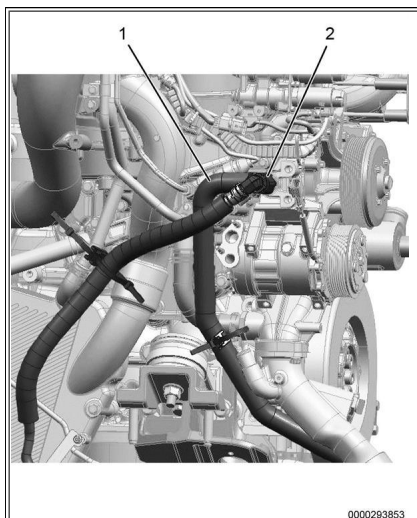
Figure 25: SCR Equipped Water Bypass Hose.
