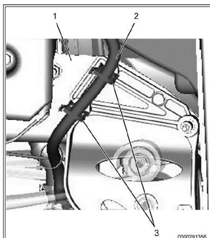
Figure 19: Frame Mounted Heater Hose Routing.
