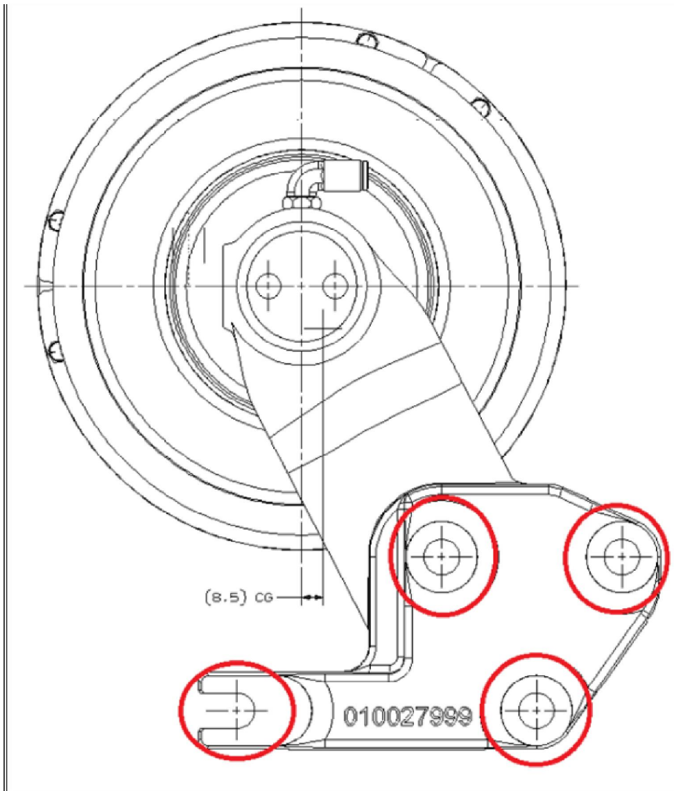
Figure 1: Fan Hub Bracket
