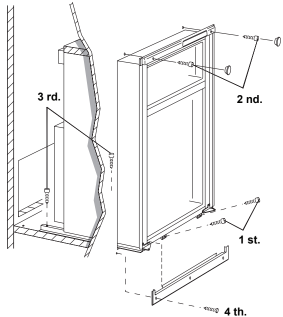
FIG 15 - SECURING RM2620 & RM2820
