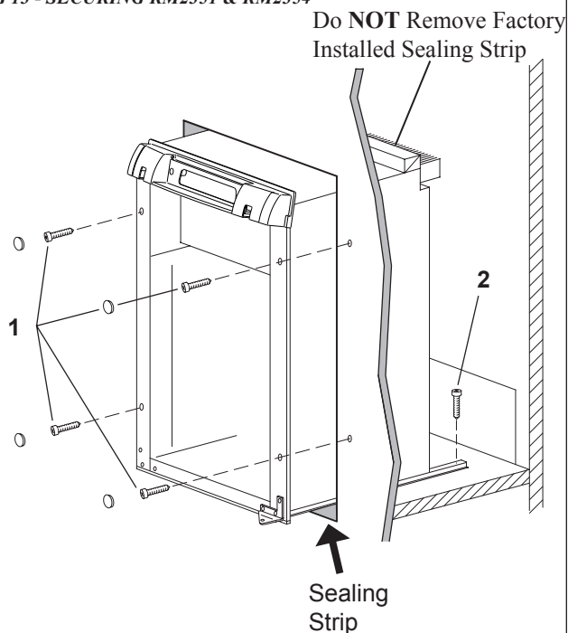
FIG 13 - SECURING RM2351 & RM2354
