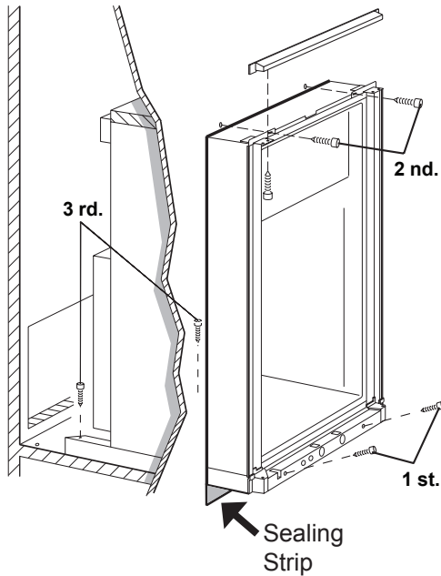
FIG 14 - SECURING RM2410 & RM2510
