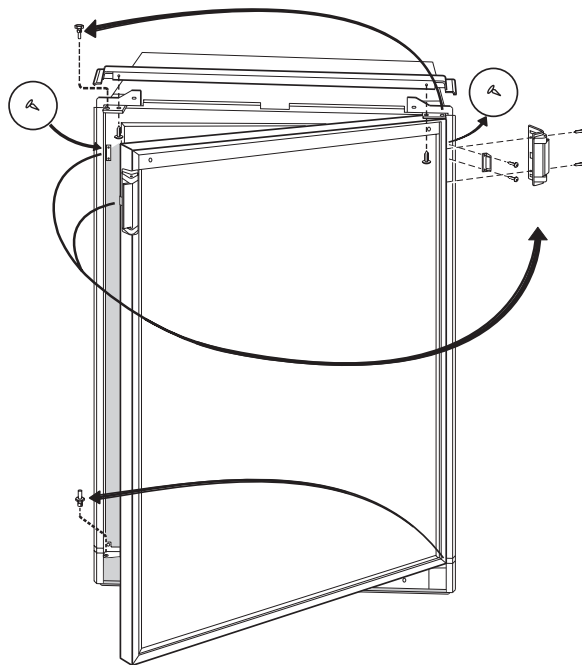
FIG 19 - RM2410 & RM2510, REVERSING THE DOOR SWING
