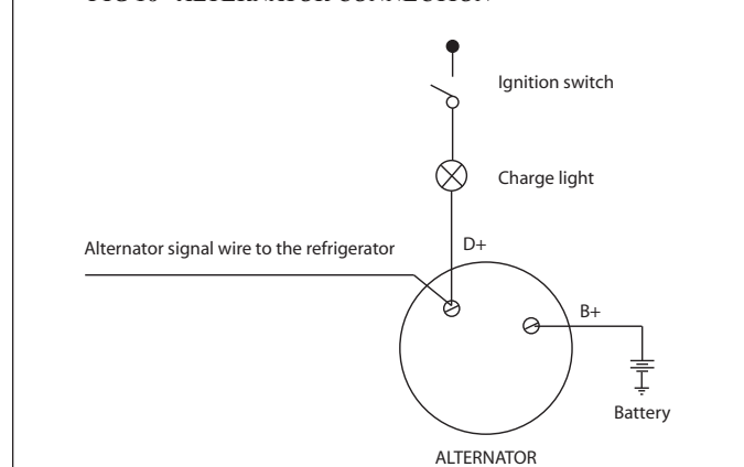
FIG 18 - ALTERNATOR CONNECTION
