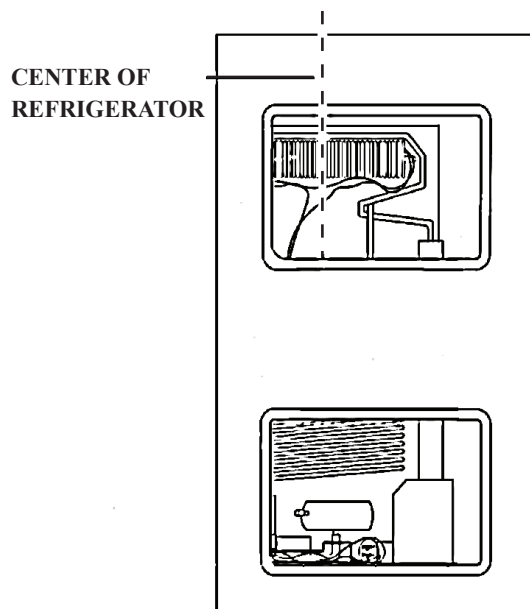
FIG 8 - OFFSET VENT UPPER AND LOWER SIDE VENT
