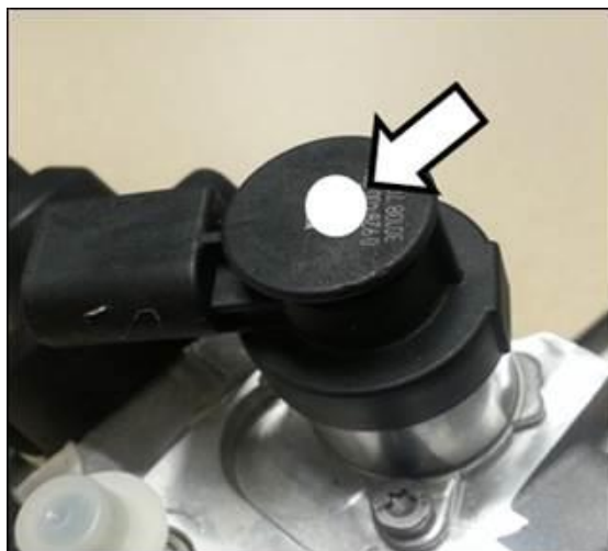
Figure 6. White dot on N290 fuel metering valve.
