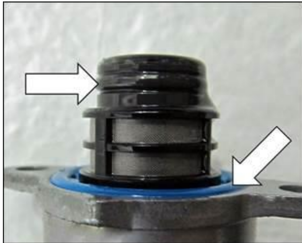
Figure 5. N290 fuel metering valve O-rings.
