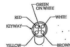
VIEW "D-D" TO R/S REAR BRANCH SCALE: 3/4
