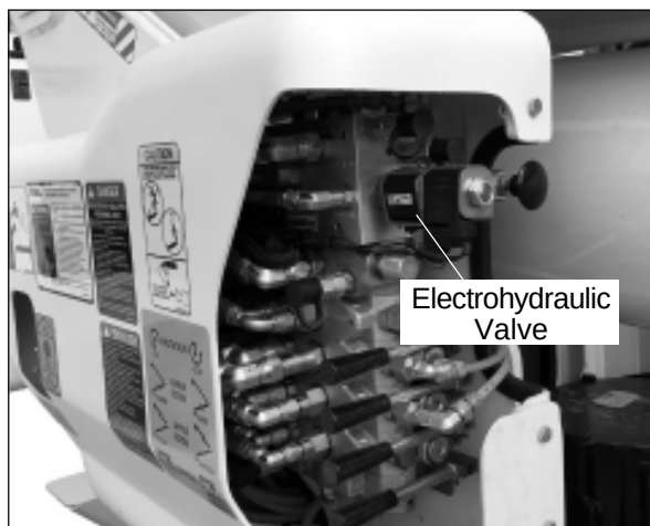
Figure 1 — Electrohydraulic Valve
