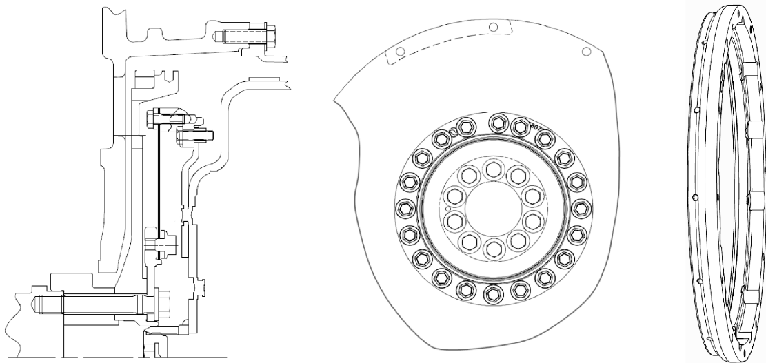
Figure 2. 29558081 Adaptation Kit (left and center) 29558082 Flexplate Adapter (right)
