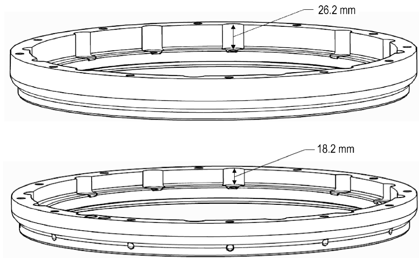
Figure 3. 29545926 Flexplate Adapter (top) 29558082 Flexplate Adapter (bottom)
