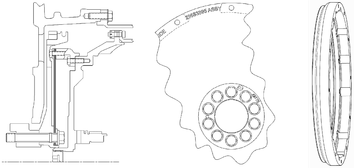
Figure 1. 29553895 Adaptation Kit (left and center) 29545926 Flexplate Adapter (right)
