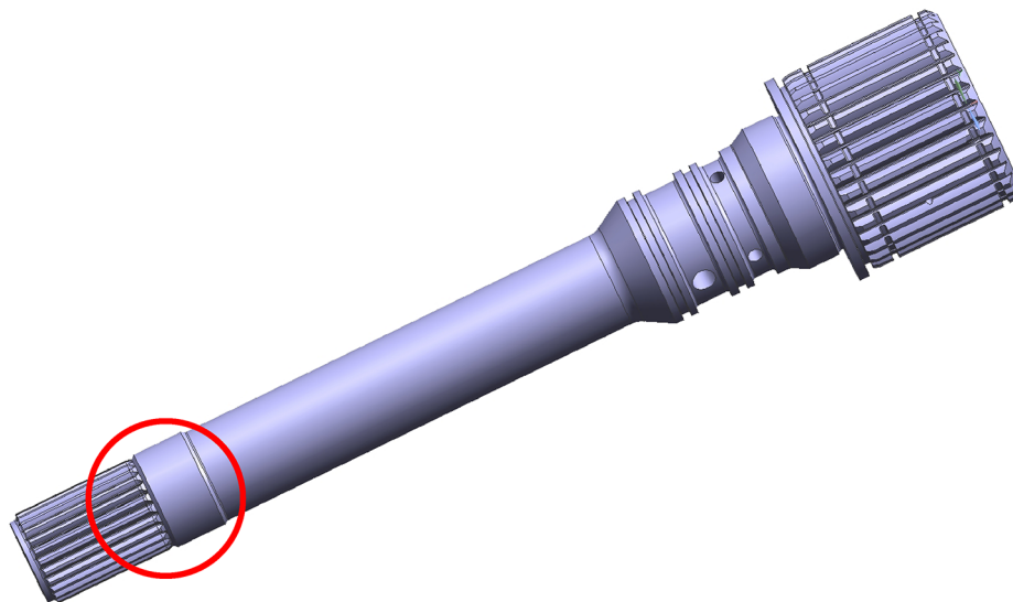
Figure 3. Current Turbine Shaft Without Undercut (P/N 29558949)
