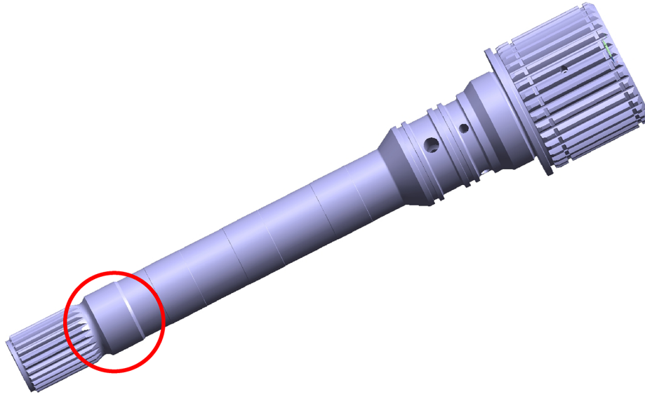
Figure 2. Former Turbine Shaft With Undercut (P/N 29548947)
