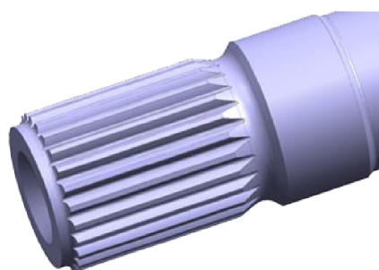
FORMER With Undercut (P/N 29548947)
