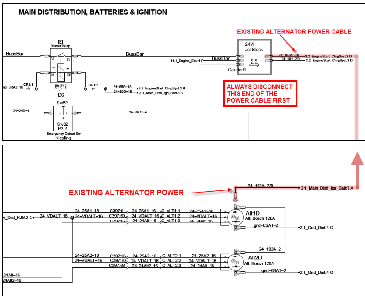
FIGURE 11: ALTERNATOR POWER CABLE
