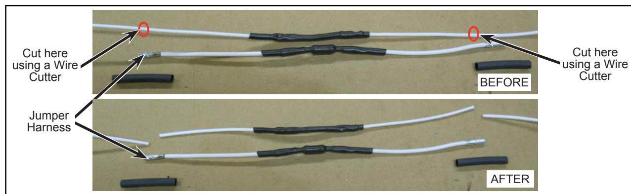
Figure 6 - Typical View of Jumper Harness
