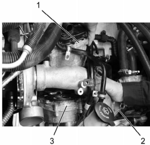
Figure 22: CCOS Housing
