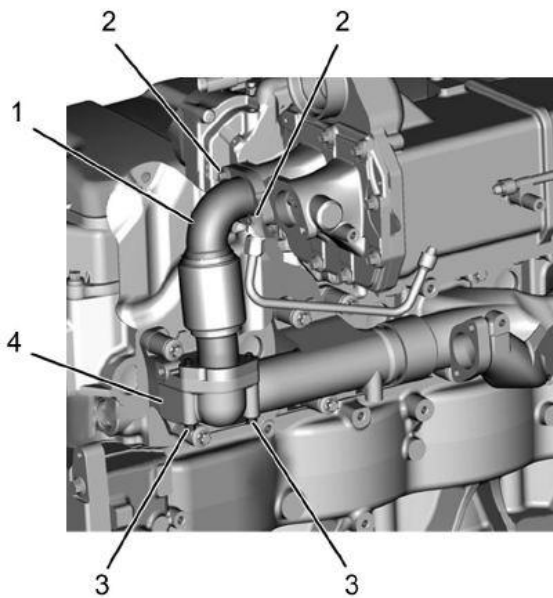
Figure 14: Inboard EGR Inlet Tube
