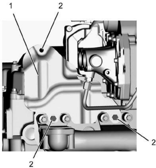
Figure 4: EGR Heat Shield
