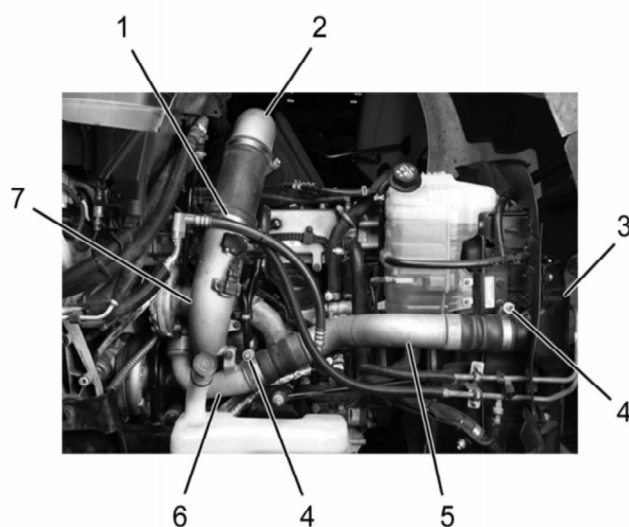
Figure 17: HP Turbocharger Connections
