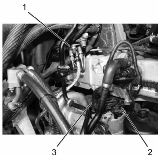
Figure 20: Air Control Valve
