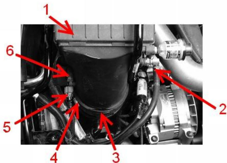
Figure 27: MAF Sensor and Air Compressor Inlet Hose
